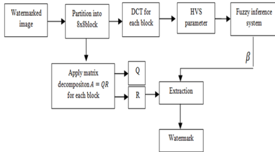
Fig. 2: Block Diagram of The Extraction Algorithm
