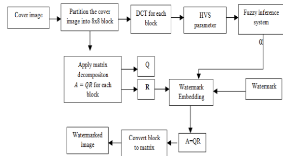
Fig. 1: Block Diagram of The Embedding Algorithm
